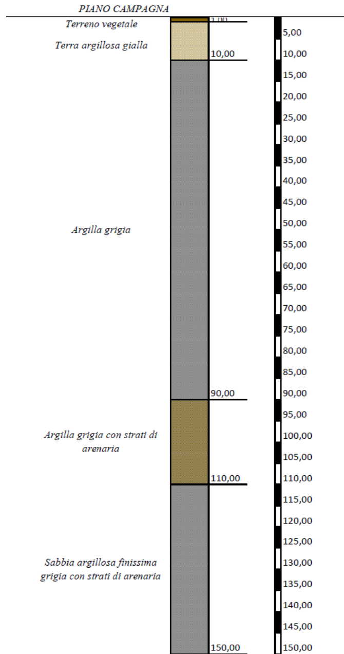
Figure 14 Stratigraphy of the ground
