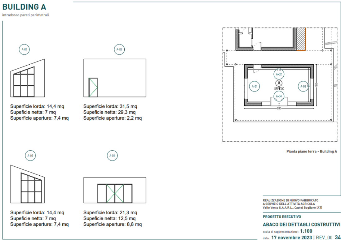
Figure 24 Building A structure
