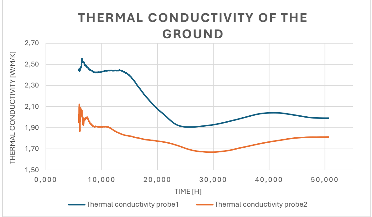
Figure 19 Conductivity of the ground with respect the time
