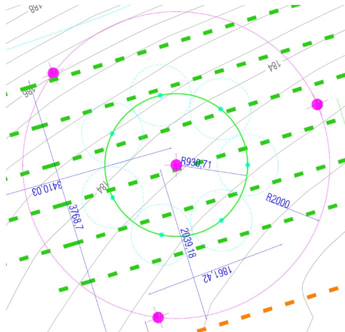
Figure 38 Boreholes layout of the BTES
