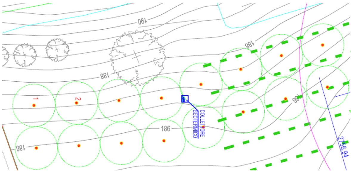
Figure 32 BHE disposition
