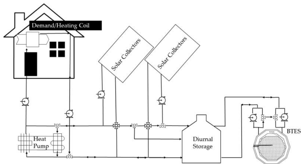
Figure 36 Concept diagram of BTES connected with solar collector and GSHP
