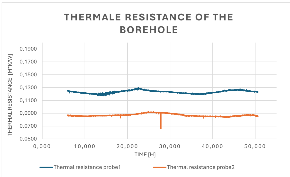
Figure 20 Thermal resistance of the probe with respect time
