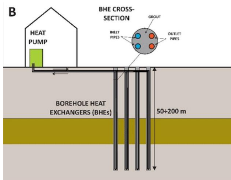
Figure 6 representation of a vertical closed loop system
