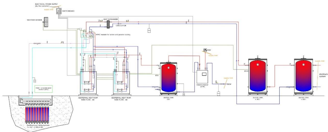
Figure 33 Scheme of the plant, Geonovis 2024
