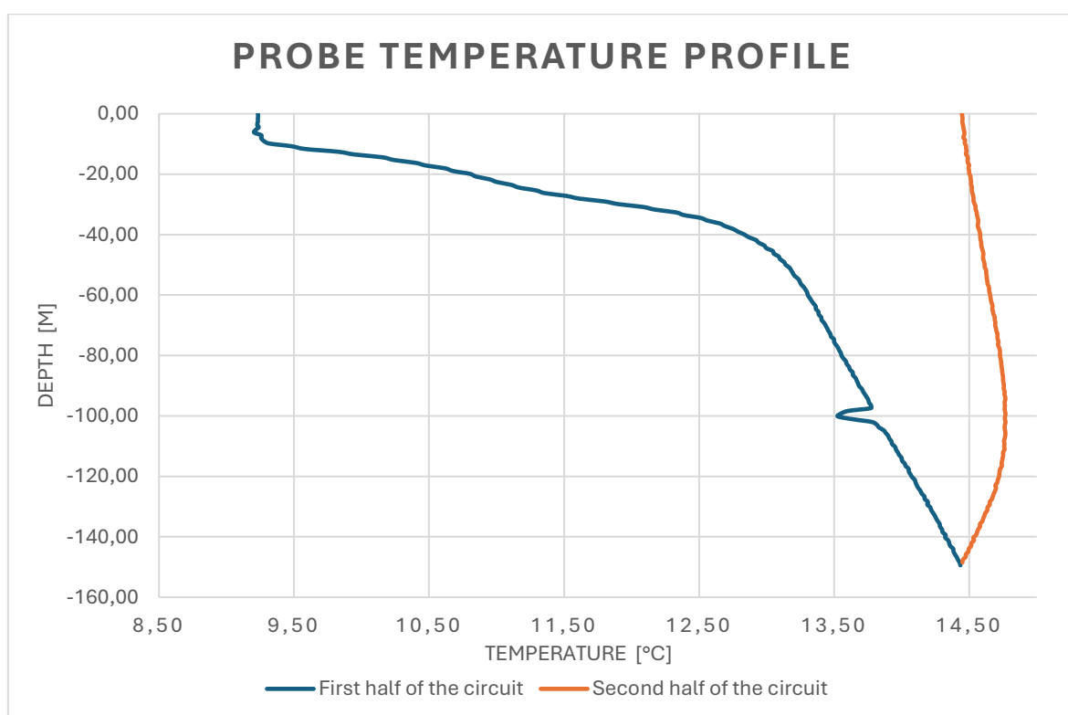
Figure 16 Temperature profile of two half of the circuit
