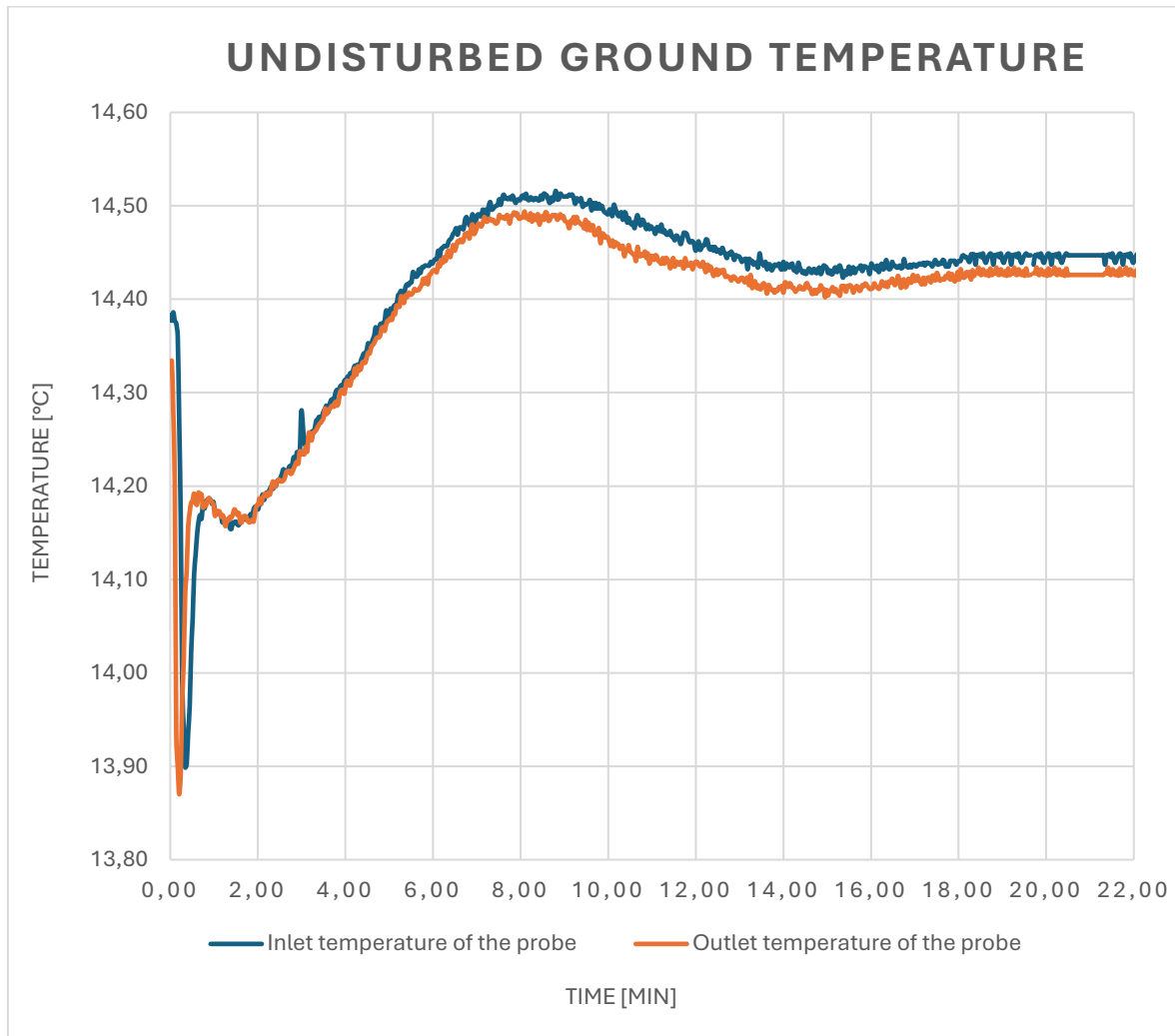
Figure 17 Undisturbed temperature of the ground
