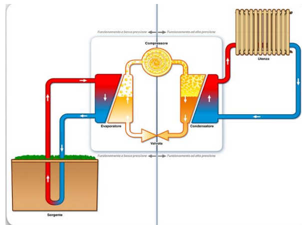
Figure 9 Operating scheme of an heat pump
