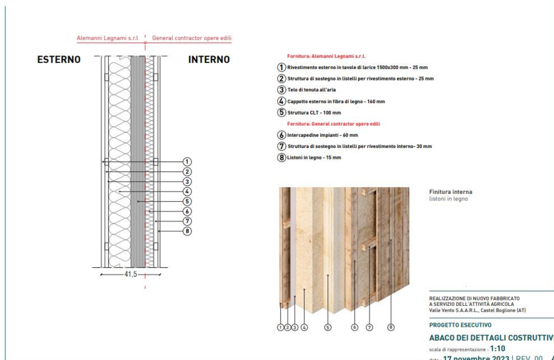
Figure 25 Stratigraphy of the walls
