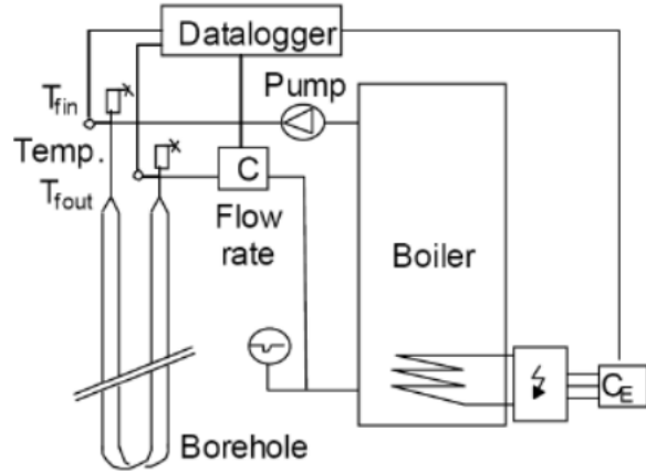
Figure 18 Scheme of operation of the TRT
