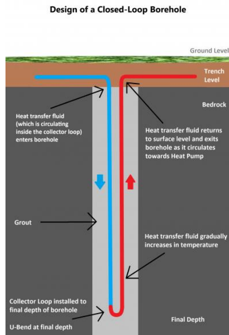
Figure 8 Design of a closed-loop borehole
